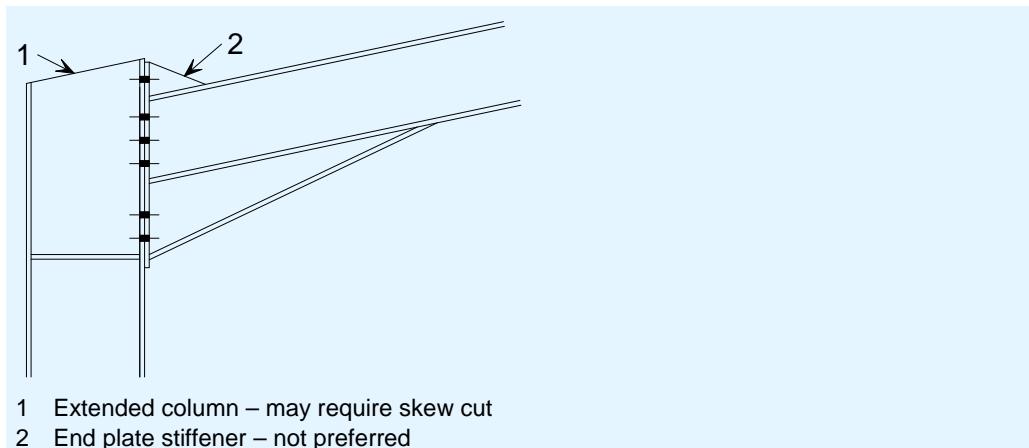
Figure 3.3 Extended end plate connection
