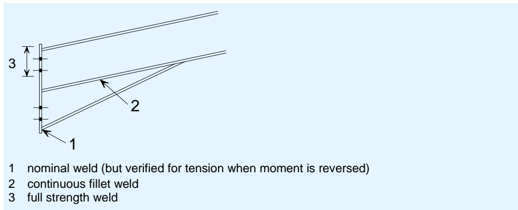
Figure 3.6 Haunch welds
